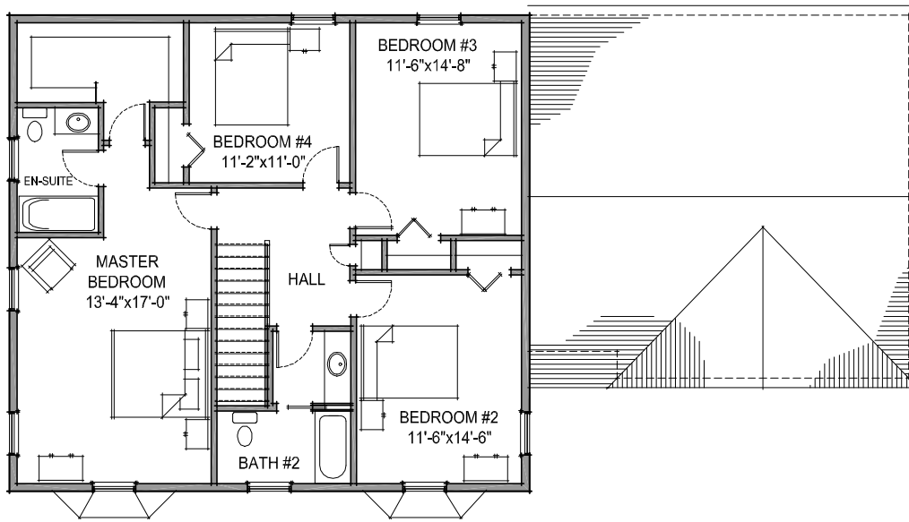
FIRST FLOOR PLAN 1,190 SQ. FT. (INC. GARAGE)
